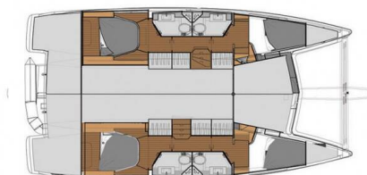
Lucia 40 4-cabin layout
